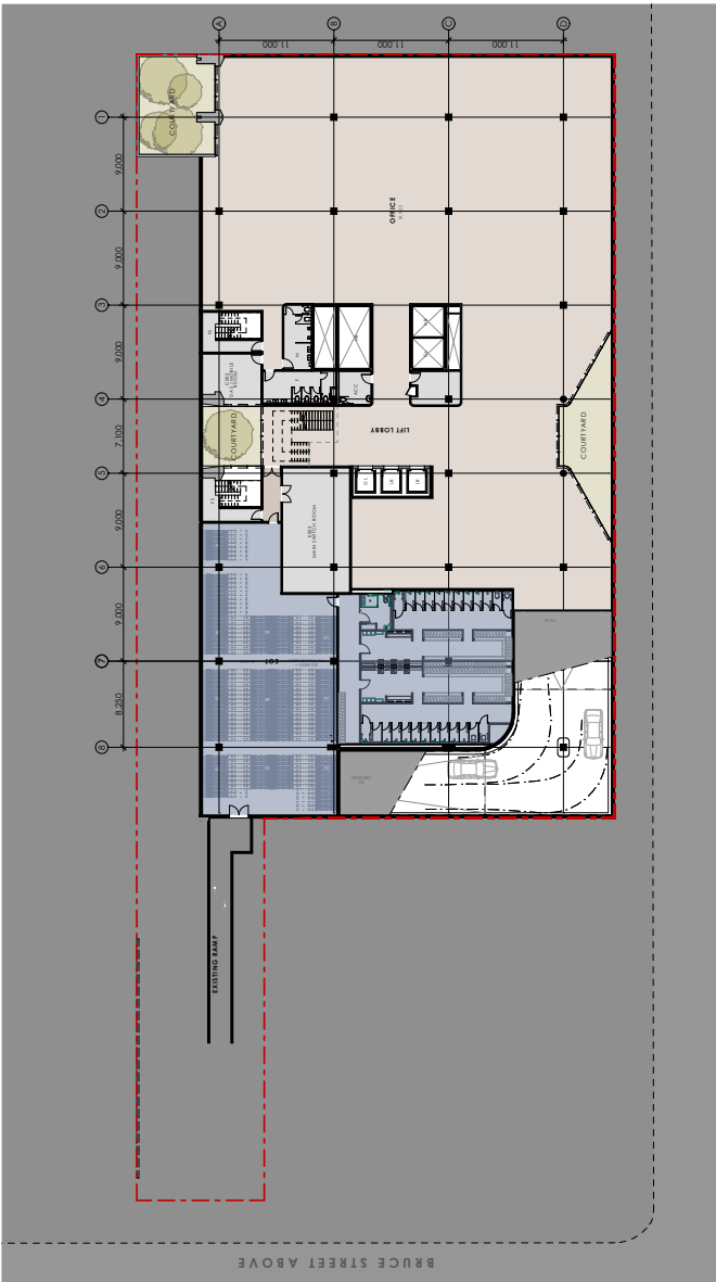
LOWER GROUND End of Trip Facilities, Tenant Space, NLA: 1505 M 2
