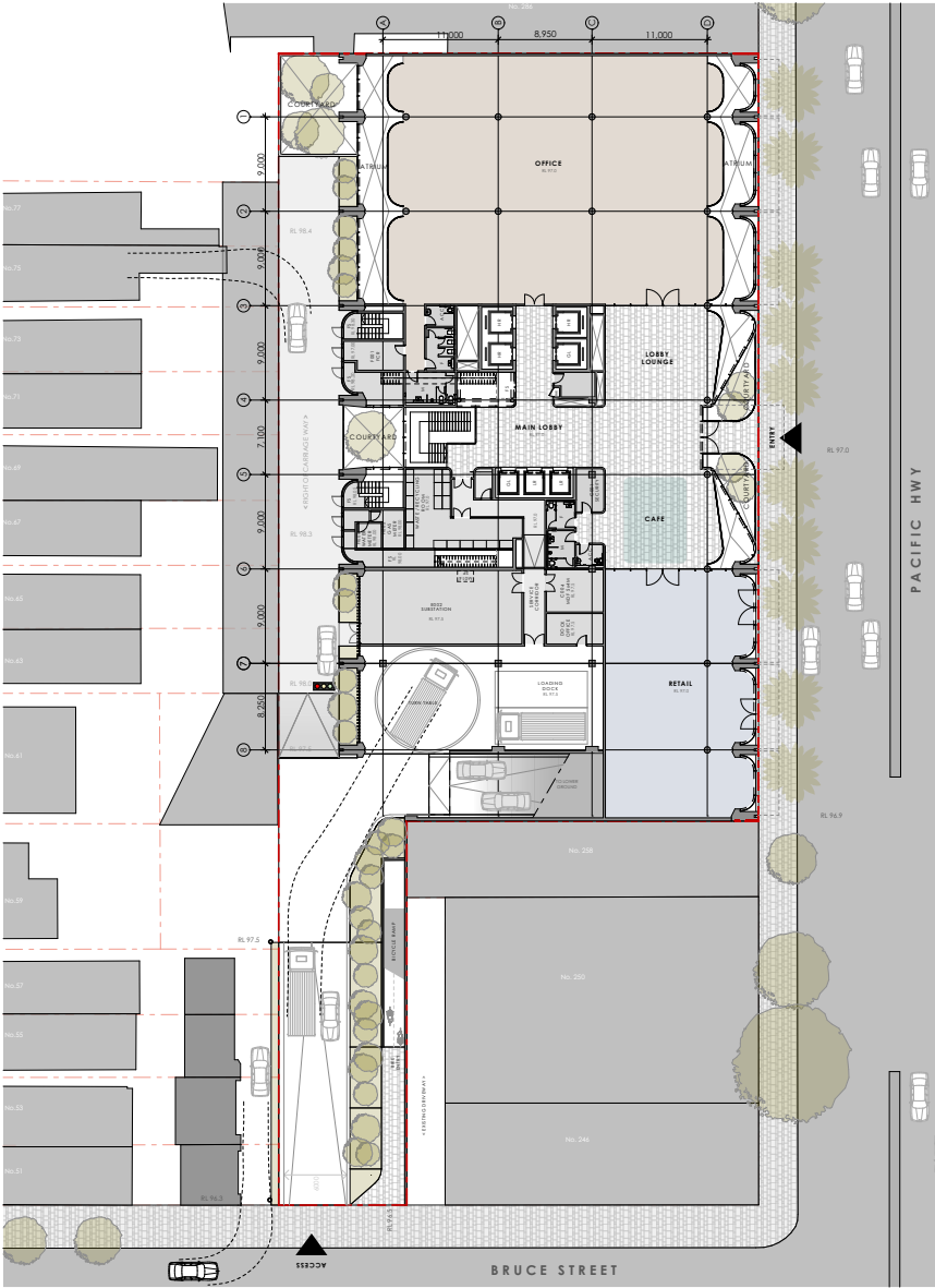
GROUND Main access of Pacific Highway, Lobby with Cafe, Retail, Tenant Space Main Building, GFA: 1,535 M 2 , Parking and Loading Entry of Bruce Street
